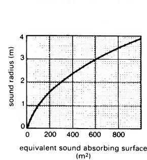
⑥ Sound radius and sound absorbing capability of a room
